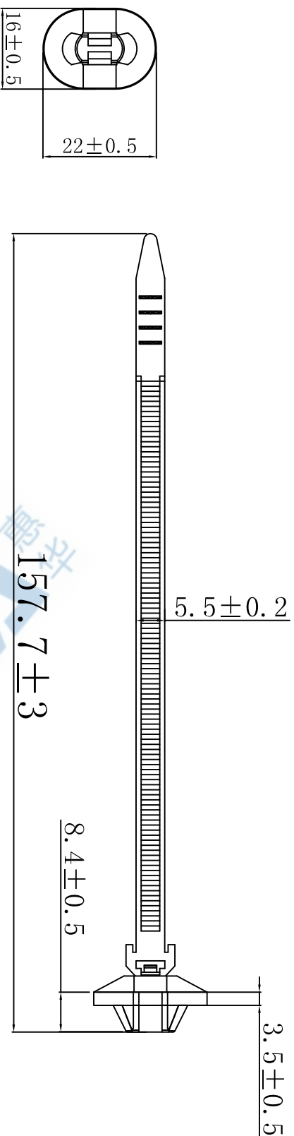
View Without Seal/ 不带海绵垫视图
